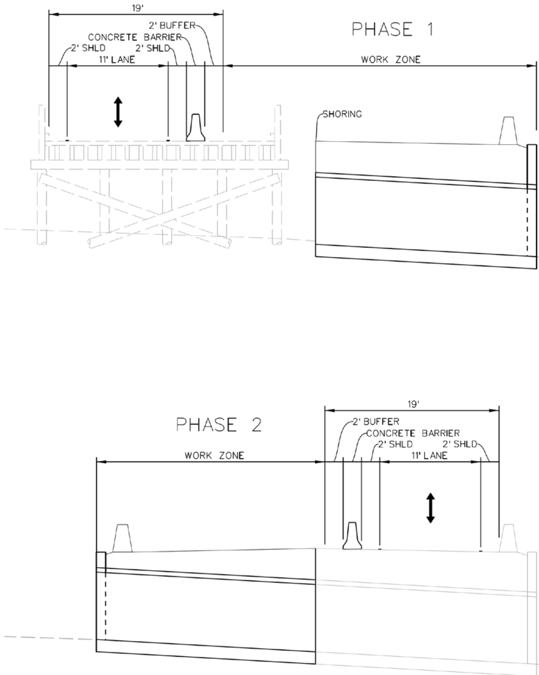
Figure 2: Single Lane – Two Way Phasing
